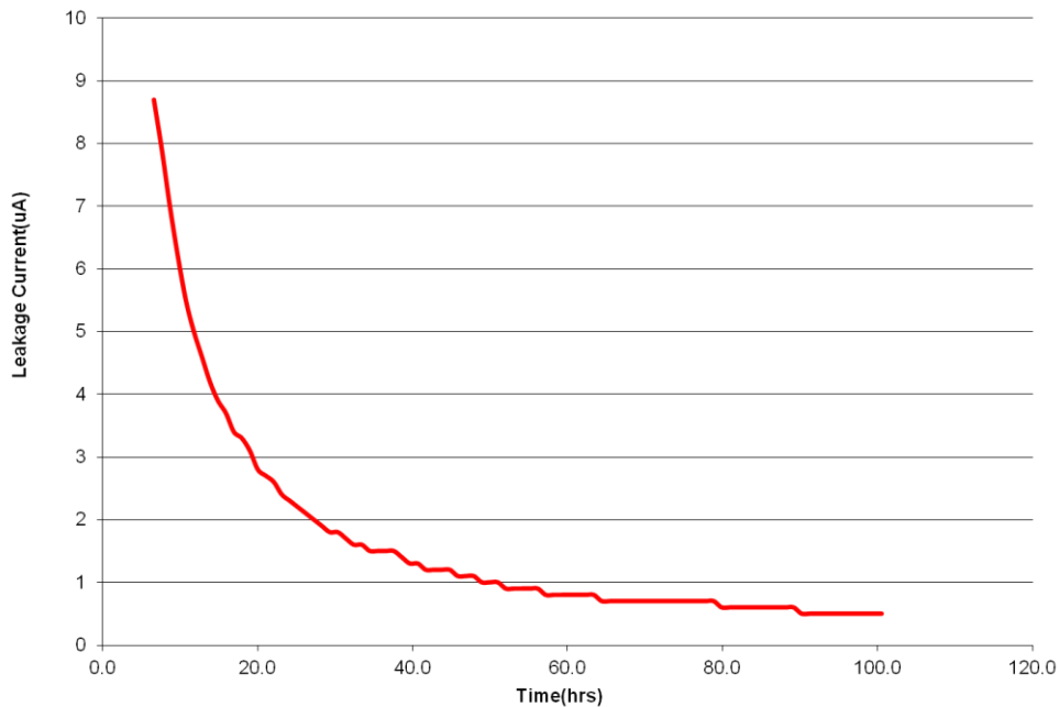
Fig 10: Leakage Current
