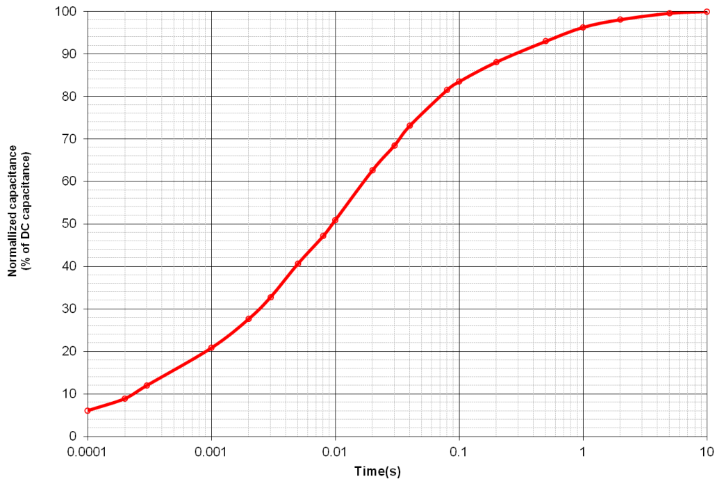
Figure 4: Effective Capacitance
